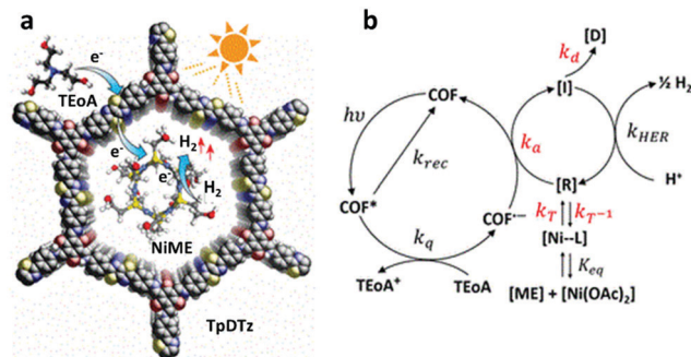
Fig. 12 (a) Schematic illustration of photocatalytic \text{H}_2 evolution. (b) The proposed kinetic steps of the photocatalytic \text{H}_2 evolution reaction with TpDTz COF and NiME cluster cocatalyst. [Ni-L] denotes a ligand-coordinated co-catalyst state which is attained fast compared to the [R] state, [R] denotes the catalyst resting state, which is catalytically active nickel cluster species, [D] denotes the deactivated species, and [I] denotes an intermediate reduced catalyst species able to run the HER step. Reproduced with permission from ref. 123. Copyright 2019, American Chemical Society.
