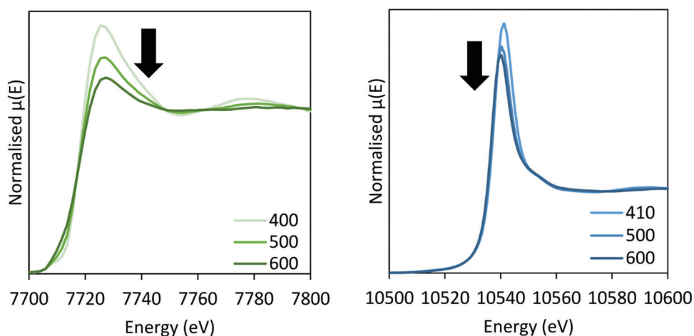
Fig. 11 XANES of the CoRe-gel during ammonia decomposition at the Co K-edge (left) and Re L_{III} -edge (right) between 400\text{--}600\text{ }^\circ\text{C} in 5\%\text{ }NH_3 .
