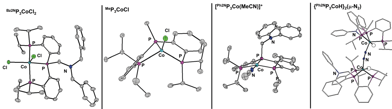
Fig. 1 50% thermal ellipsoid plot of several complexes. All hydrogen atoms not located in the difference map are removed for clarity. Only the cation of [(\text{Ph2N}_3\text{P}_3\text{Co}(\text{MeCN}))][\text{BARF}] is shown.
