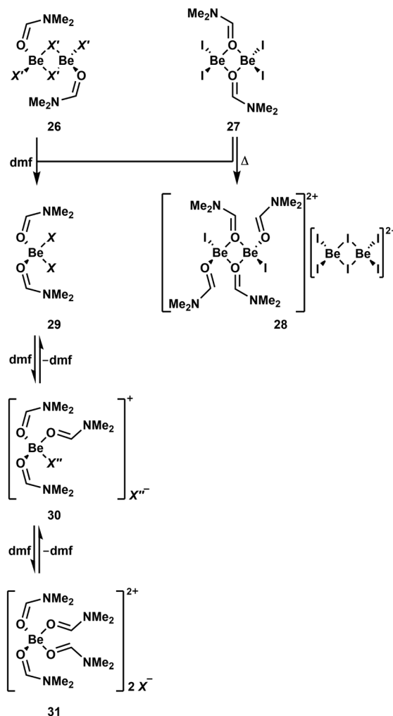
Scheme 5 Various N,N -dimethylformamide (dmfm) adducts of the beryllium halides. X = Cl (a), Br (b), I (c); X' = Cl (a), Br (b); X'' = Cl (a), I (c). 90,91
