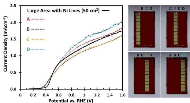
Fig. 4 AM1.5G J – V curves for the \text{W:BiVO}_4 photoanodes with Ni lines, measured on 4 different areas of the sample (right, A–D) to determine the uniformity of the photocurrent across the large area sample, with an electrolyte containing 0.5 \text{ M Na}_2\text{SO}_3 and 0.1 \text{ M KPi} buffer of pH 7.
