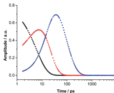
Fig. 6 (Top) Differential absorption spectra obtained by femtosecond transient absorption pump-probe experiments (550 nm, 400 nJ) of (\text{TCBD-aniline})_3\text{-SubPc-(TCBD-aniline)} ( 2 ) ( 3 \times 10^{-5} \text{ M} ) in argon-saturated anisole with several time delays between 1 to 7500 ps. (Middle) Deconvoluted evolution associated spectra and (bottom) associated time-dependent amplitudes obtained via global analysis in GloTarAn monitoring formation and decay kinetics.
