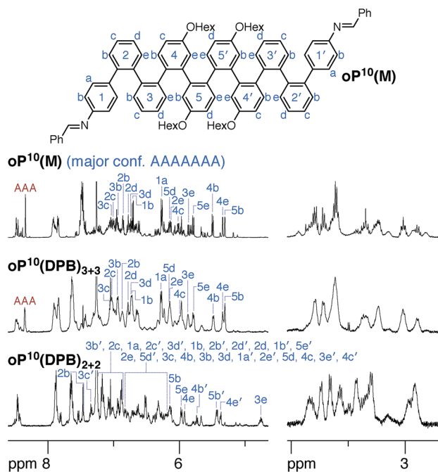
Fig. 8 ^1\text{H} NMR spectra (500 MHz, 0 °C) of \text{oP}^{10}(\text{M}) , \text{oP}^{10}(\text{DPB})_{2+2} , and \text{oP}^{10}(\text{DPB})_{3+3} . ^1\text{H} assignments for the major conformers are shown (blue). For \text{oP}^{10}(\text{DPB})_{2+2} , the assignments that are grouped together are listed in order from least- to most-shielded; chemical shifts for a minor conformation were also assigned (not shown).
