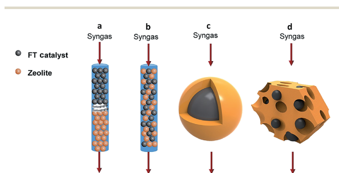
Fig. 5 Integration manners of bifunctional catalysts consisting of a FT catalyst component and zeolite: (a) dual-bed reactor, (b) physically mixing, (c) core-shell structure, (d) loading of FT metal particles on the zeolite. Reprinted from ref. 7 with permission from Elsevier.
