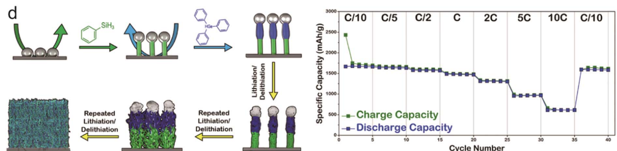
Fig. 4 Si-based composite materials as anodes: Si/graphite composites, (a–c) schematic of the procedures for the fabrication of SEAG. Reproduced with permission. 56 Copyright (2017) Nature Publishing Group (a). Schematic gelation process and a picture as well as the model of the Si@C@Cu composite. Reproduced with permission. 57 Copyright (2019) American Chemical Society (b). Schematic illustration of the synthesis of B–Si/CNT. Reproduced with permission. 58 Copyright (2019) American Chemical Society (c). Si–metal alloy, (d) overview of the synthetic protocol used to prepare Sn-seeded Si–Ge hNWs directly from current collectors. Charge and discharge capacities ( \text{mA h g}^{-1} ) demonstrated at different current rates. Reproduced with permission. 29 Copyright (2018) American Chemical Society (d).
