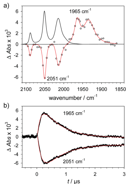
Fig. 5 (a) Transient IR spectrum 0.3 \mu\text{s} after excitation (O, \color{red}\dashrightarrow ) and normalized IR spectrum of the starting state ( \color{black}\text{---} ) for formation of \mathbf{1H} by reduction of \mathbf{1H}^+ (obtained by protonation of \mathbf{1} with 2.6 mM \text{Cl}_2\text{BSA} ) with flash-quench generated [\text{Ru}(\text{dmb})_3]^+ in acetonitrile. (b) Kinetic traces ( \color{black}\cdots ) and fits ( \color{red}\text{---} ) monitoring pseudo-first order formation of \mathbf{1H} ( 1965\text{ cm}^{-1} ) and bleach of \mathbf{1H}^+ ( 2051\text{ cm}^{-1} ) followed by pseudo-first order decay of \mathbf{1H} by protonation with \text{Cl}_2\text{BSA} and charge recombination with \text{TTF}^+ .
