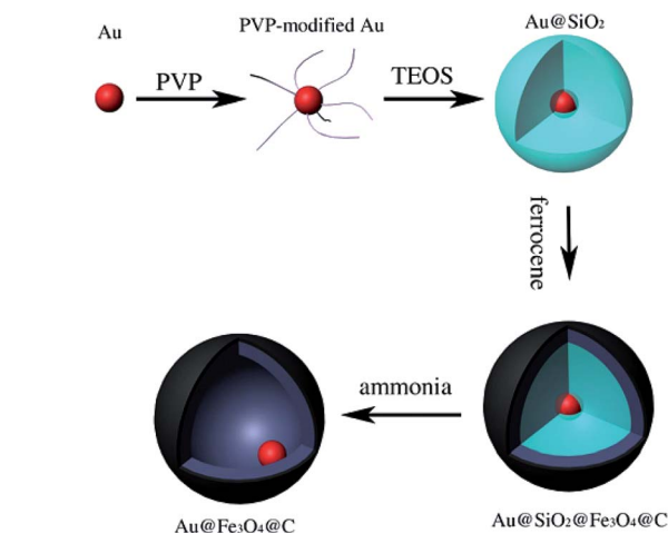
Fig. 8 Schematic of the preparation procedure of yolk-type Au@Fe 3 O 4 @C. 80
