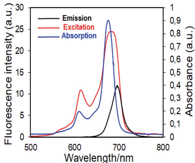
Fig. 6 Electronic absorption, fluorescence emission and excitation spectra of 4 in DMSO. (Excitation wavelength = 697 nm.)
