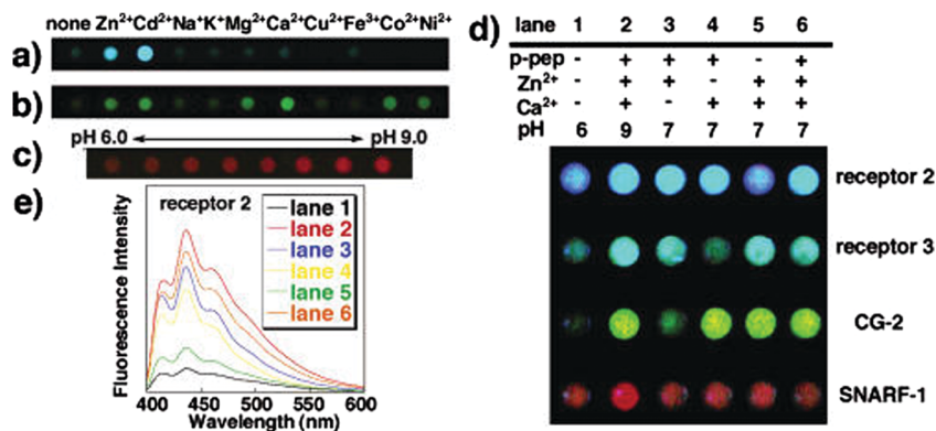
Fig. 13 Photographs of sensing patterns of semi-wet chemo sensor chip made from hydrogels containing different receptors and the corresponding fluorescence emissive spots in reaction to mixed solutions containing the various analyte concentrations. 74
