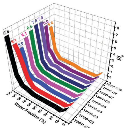
Fig. 3 Plot of the ratio of the maximum fluorescence intensity ( I/I_0 ) of the nine TPPP derivatives vs. the water fraction.
