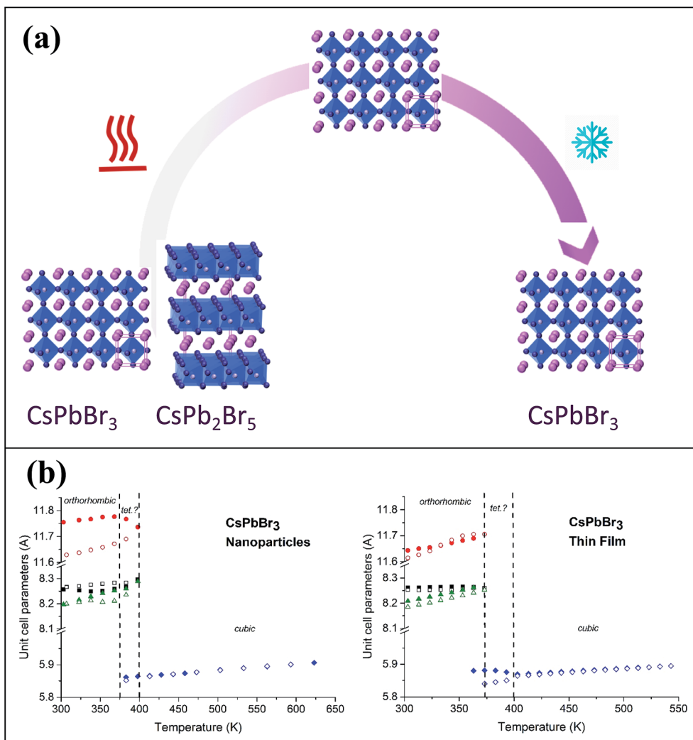
Fig. 3 (a) Schematic illustration of the process described in this work. On heating the \text{CsPbBr}_3 thin films to 623 K, the \text{CsPb}_2\text{Br}_5 disappears and pure \text{CsPbBr}_3 remains when cooling down to room temperature. (b) Cell parameters as a function of temperature for (left) NPs and (right) thin films. Triangles, squares and circles correspond to the a , b and c unit cell parameters, respectively. Closed and open symbols correspond to the heating and cooling sequence, respectively. The uncertainty of the cell value is contained within each symbol. 'tet' corresponds to tetragonal.
