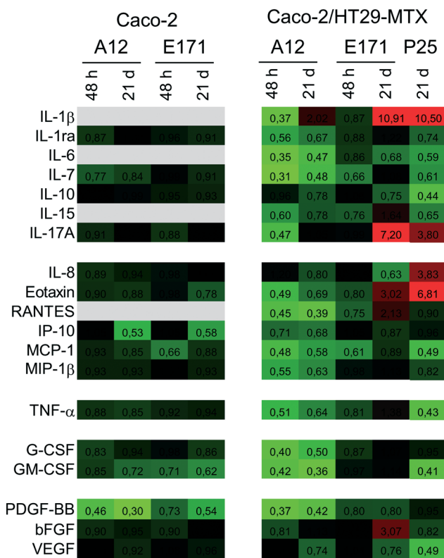
Fig. 3 E171 and TiO 2 -NPs trigger an inflammatory response. The BioPlex MagPix™ technology was used to screen cells for the expression of the following 27 cytokines: interleukins (IL-1β, 2, 4, 5, 6, 7, 9, 10, 12, 13, 15, 17A), chemokines (IL-8, eotaxin, RANTES, IP-10, MCP-1, MIP-1β, and MIP-1α, the latter was under the LQ in both cell models and is therefore absent from this heat map), tumor necrosis factor family (TNF-α), interferon (IFN-γ), colony stimulating factors (G-CSF and GM-CSF), and growth factors (PDGF-BB, basic FGF, and VEGF). Caco-2 and Caco-2/HT29-MTX were exposed to 50 µg per mL of E171 or A12, either acutely for 48 h or repeatedly twice a week for 21 days. In addition, the secretion of these cytokines was measured in Caco-2/HT29-MTX co-cultures repeatedly exposed to 50 µg per mL of P25. Results represent fold-change of protein concentration in exposed cells vs. control cells. They are presented as a heat map, with the color scale ranging from light green to black (fold-change: 0 to 1) and from black to light red (fold-change: 1 to 11); gray: below the limit of detection. Numbers indicated in boxes correspond to fold-changes.
