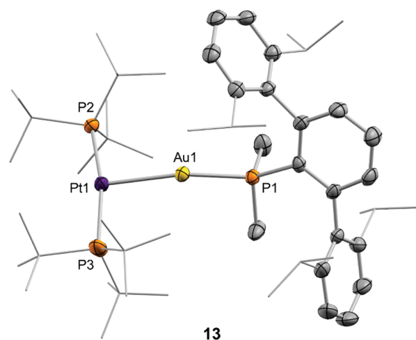
Fig. 7 ORTEP diagram of the cation of complex 13 ; hydrogen atoms, half molecule of [(\text{PMe}_2\text{Ar}^{\text{Dipp}})_2\text{Au}]^+ and triflimide anions are excluded for clarity and thermal ellipsoids are set at 50% probability. tert -Butyl and iso-propyl substituents have been drawn in wireframe format.
