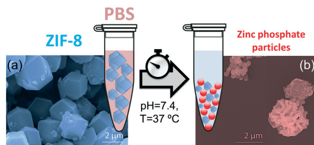
Fig. 1 Incubation process of ZIF-8 particles in phosphate buffered saline media (PBS) under physiological conditions of pH (7.4) and temperature (37 °C). (a) SEM image of as-synthesized micro-ZIF-8 particles. (b) SEM image of micro-ZIF-8 particles after being soaked in PBS for 24 h.
