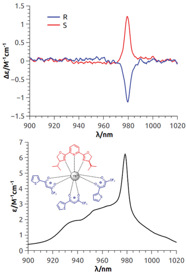
Fig. 3 Top: NIR-ECDA spectra of both the enantiomers of \text{Yb}(\text{TTA})_3\text{PrPyBox} ; bottom: total NIR absorption. The spectra are measured in 7 mM \text{CH}_2\text{Cl}_2 solution (room temperature).
