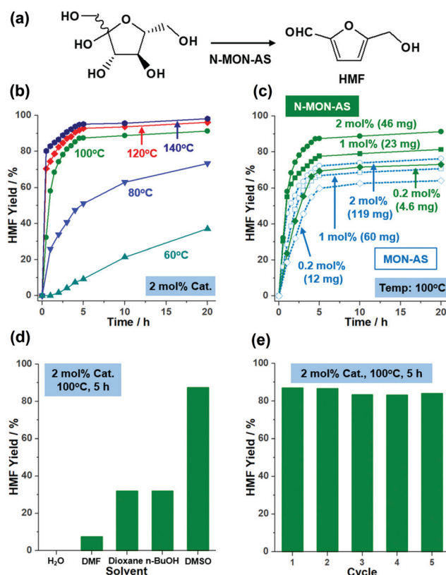
Fig. 4 (a) A scheme of fructose conversion to HMF. (b) Temperature-dependent catalytic performance of N-MON-AS. (c) Comparison of the catalytic performance of MON-AS (0.284 mmol SO 3 H per g) and N-MON-AS (0.731 mmol SO 3 H per g). (d) Solvent-dependent catalytic performance and (e) recyclability of N-MON-AS.
