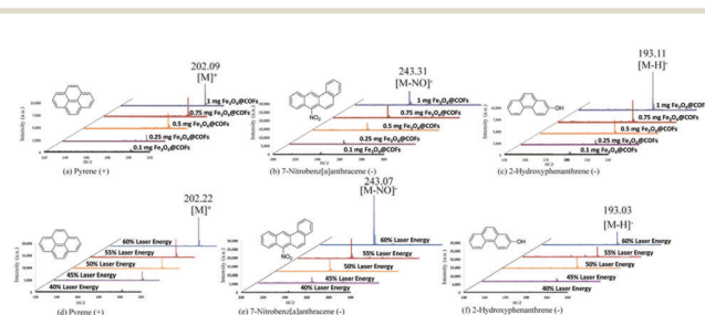
Fig. 2 Optimization of matrix dosage (a–c, laser energy: 50%) and laser energy (d–f, matrix dosage: 1 mg) with 100 ng of a single standard.
