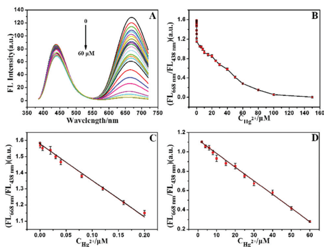
Fig. 2 (A) Fluorescence emission spectra of AuNCs/MIL-68(In)-NH 2 /Cys in the presence of Hg 2+ with different concentrations (0, 2 × 10 -4 , 5 × 10 -3 , 0.02, 0.03, 0.04, 0.08, 0.12, 0.16, 0.2, 2, 4, 6, 8, 10, 15, 20, 25, 30, 40, 50 and 60 μM). (B) Plot of the fluorescence intensity ratio (FL 668 nm /FL 438 nm ) versus the concentration of Hg 2+ . (C) The linear relationship between FL 668 nm /FL 438 nm and the concentration of Hg 2+ ranging from 20 pM to 0.2 μM. (D) The linear relationship between FL 668 nm /FL 438 nm and the concentration of Hg 2+ ranging from 0.2 μM to 60 μM. The error bars represent the standard deviation of three measurements (λ ex = 370 nm, slit: 5/5 nm).
