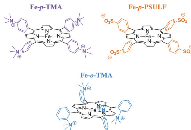
Fig. 2 Iron tetraphenylporphyrin derivatives with positive and negative charges used for electrocatalytic reduction of CO 2 to CO. Reprinted with permission from ref. 88. Copyright 2016, American Chemical Society.
