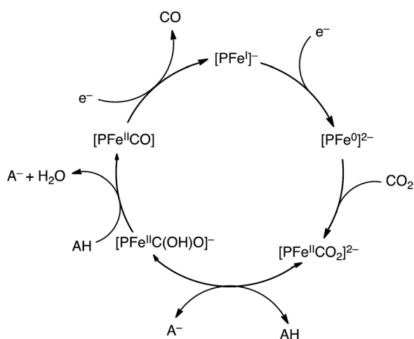
Scheme 3 Catalytic cycle for two-electron reduction of CO 2 to CO with an iron porphyrin ([PFe] − ). 84
