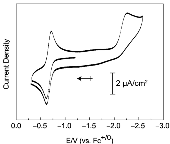
Fig. 4 Cyclic voltammogram of [\text{Mn}^{\text{IV}}(\text{O})(\text{ditox})_3][\text{K}(15\text{-C-5})_2] ( 3 ) in THF/[TBA][PF 6 ].
