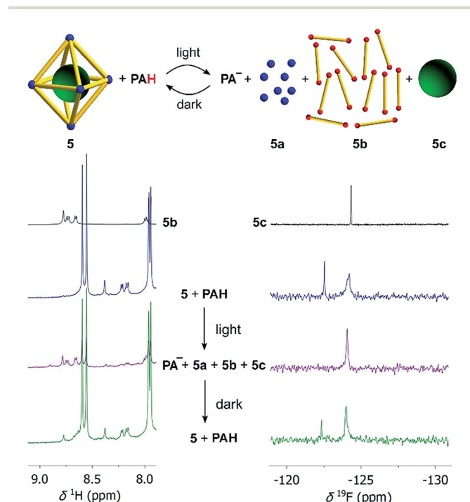
Scheme 4 Irradiation of a mixture of cage 5 ( 10 \mu M ), NaCl ( 60 \mu M ), and the photoacid PAH (8 equiv. with respect to each bipyridyl ligand) in CD_3CN/D_2O (8 : 2) by violet light results in disassembly of the cage and liberation of the [B(p-C_6H_4F)_4]^- guest (green ball) as evidenced by the ^1H NMR (left) and ^{19}F NMR spectra (right). Details about the bridging ligand (yellow) are given in the ESI.†
