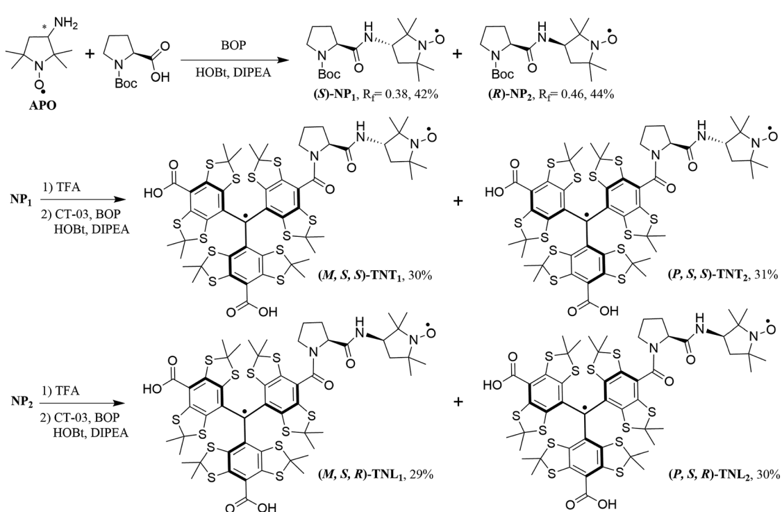
Scheme 1 Synthesis of the four enantiomerically pure diastereoisomers of TN biradicals. M/P represents the helices of the trityl radical, while R/S indicates the configurations of L -proline and the nitroxide APO.
