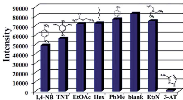
Fig. 3 Fluorescence responses of the complex with different organic molecules. ( 1 \times 10^{-3} mol L ^{-1} , excited at 365 nm).
