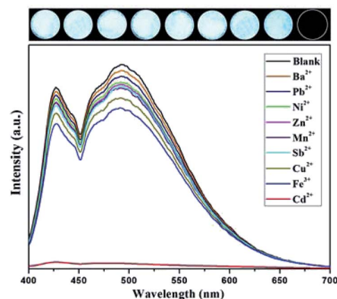
Fig. 4 Fluorescence responses of the complex with different toxic metal ions ( 1 \times 10^{-3} mol L -1 , excited at 365 nm).
