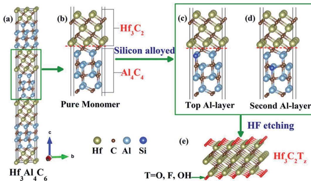
Fig. 2 Schematic illustration of the synthesis of Hf_3C_2T_z MXene from nanolaminated phase Hf_3[Al(Si)]_4C_6 . (a) Structure of Hf_3[Al(Si)]_4C_6 , (b) structure of pure Hf_3Al_4C_6 monomer, (c) and (d) structure of two Hf_3Al_4C_6 monomers with different silicon alloying, and (e) side view of Hf_3C_2T_z MXene. Reprinted with permission of ref. 36 Copyright 2017 American Chemical Society.
