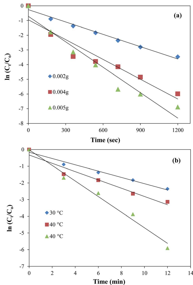
Fig. 8 Dependence of k_{\text{app}} on (a) the amount of catalyst at 30^\circ\text{C} and (b) temperature. Reaction conditions; 0.5 mM aqueous solution of 2-nitroaniline = 50 ml, \text{NaBH}_4 = 0.1 g, graphene oxide-gold catalyst = 5 mg, 100 rpm.
