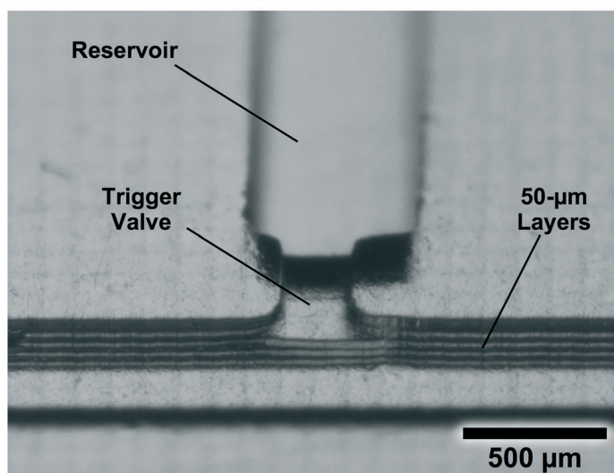
Fig. 13 Rapid prototyping of capillary components and circuits using CO 2 laser cutting and 3D-printing. (A) Capillary components fabricated by CO 2 laser cutting. (i) Capillary pump, (ii) trigger valves. (B) Cross-sections of microchannels fabricated by laser cutting. Smaller microchannels (i) have a triangular Gaussian profile that reflects the shape of the laser beam, while (ii) wider microchannels have a more rectangular shape due to repeated scanning of the laser. (C) Front view of 3D-printed trigger valve showing inherent layer-by-layer structure. (D) 3D-printed mold of CC for bacteria detection showing physical realization of structures. Adapted with permission from: (A) ref. 42 © 2013 Springer-Verlag, (B) ref. 42 © 2013 Springer-Verlag Berlin Heidelberg, (C) ref. 44 © 2016 Royal Society of Chemistry, (D) ref. 45 © 2017 American Chemical Society.
