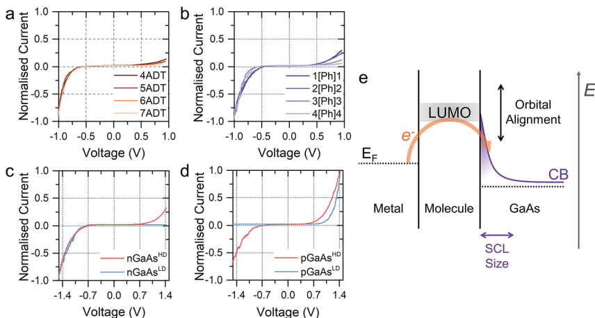
Fig. 2 (a) I – V characteristics of \alpha,\omega -alkanedithiols of increasing length on n\text{GaAs}^{\text{HD}} . (b) I – V characteristics of the \text{X[Ph]X} series on n\text{GaAs}^{\text{HD}} . (c) I – V characteristics of 5ADT on n\text{GaAs} of different doping concentration. (d) I – V characteristics of 5ADT on p\text{GaAs} of different doping concentration. (e) Band diagram for the reverse biased junction with n\text{GaAs} , where E is the electron energy. All data shown in this Figure is obtained in the dark. Note that the sense corresponding to forward bias is opposite between panel c and d. Junctions made at n -type \text{GaAs} have forward bias at negative potential, and junctions made at p -type \text{GaAs} have forward bias at positive potential.
