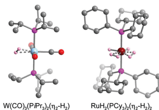
Fig. 8 Crystal structure of W(CO) 3 (PiPr 3 ) 2 (η 2 -H 2 ) (left) and RuH 2 (PCy 3 ) 2 (η 2 -H 2 ) 2 (right). 179,182 Gray, red, pink, blue, dark red, and light pink spheres represent C, O, P, W, Ru, and coordinated H atoms, respectively. Hydrogen atoms of the triphosphine ligands are omitted for clarity.
