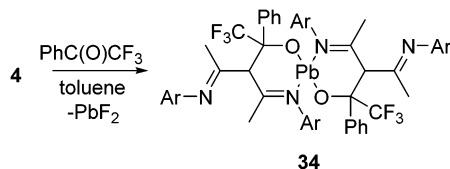
Scheme 12 The reaction of 4 with trifluoroacetophenone ( \text{Ar} = 2,6\text{-iPr}_2\text{C}_6\text{H}_3 ).
