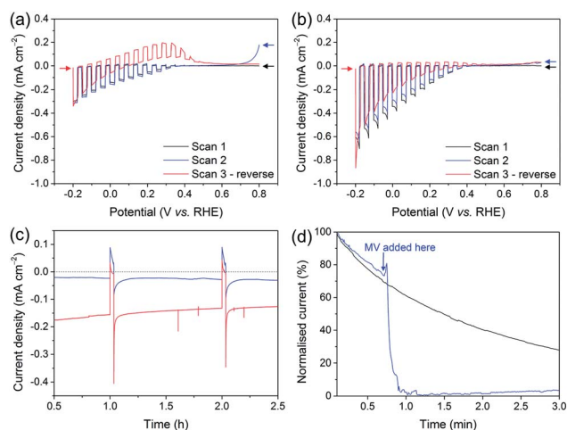
Fig. 6 LSVs under chopped illumination of (a) Si|meso \text{TiO}_2 and (b) Si|meso \text{TiO}_2 || \text{NiP} with the first two scans in cathodic direction and the third scan in anodic direction following scan reversal. Arrows indicate scanning direction for all LSVs ( v = 5 \text{ mV s}^{-1} ). (c) Enlarged view of the first two dark chops during CPP of Si|meso \text{TiO}_2 (blue) and Si|meso \text{TiO}_2 || \text{NiP} (red). (d) Chronoamperogram of Si|meso \text{TiO}_2 in the dark (normalised and given as a percentage) after being exposed to light (to charge the CB), without MV (black trace) and with MV added halfway (blue trace); E_{\text{app}} = 0.0 \text{ V vs. RHE} . Conditions: aqueous acetic acid solution (0.1 M, pH 4.5), UV-filtered simulated solar light irradiation (AM1.5G, 100 \text{ mW cm}^{-2} , \lambda > 400 \text{ nm} ), inert atmosphere, room temperature.
