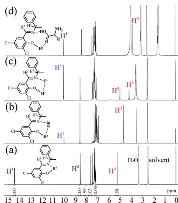
Fig. 11 ^1\text{H} NMR spectra of 3,5-Cl-diPh (a), 3,5-Cl-diPh + 100 equiv. of \text{OH}^- (b), 3,5-Cl-diPh + 100 equivalent of \text{F}^- (c), and 3,5-Cl-(R,R)-diPh + 100 equivalent of L-Arg (d) in DMSO-d 6 .
