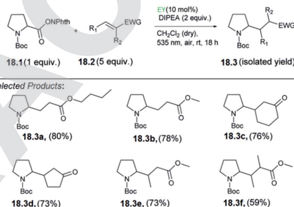
Scheme 18 Decarboxylative alkylation.
