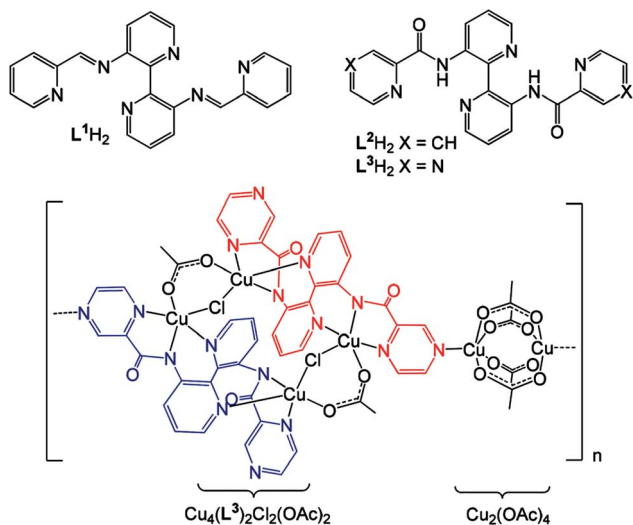
Fig. 13 (Top) Heterocyclic bis-imine and bis-amide ligands prepared from 3,3'-diamino-bipyridine. (Bottom) The molecular structure of CP comprised of a 1D arrangement of [\text{Cu}_4\text{L}_2\text{Cl}_2(\text{OAc})_2] and paddle wheel [\text{Cu}_2(\text{OAc})_4] units; for ease, the two ligands within the \text{Cu}_4 unit are shown in red and blue. [Reproduced from ref. 140 with permission from The Royal Society of Chemistry.]
