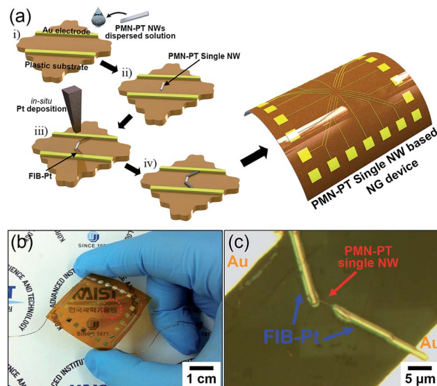
Fig. 3 (a) Schematic illustration of the overall fabrication process for a single PMN-PT NW based PEH. (b) Photograph of a flexible nano-scale PEH device connected with Cu wires. (c) PMN-PT NW connected with Au electrodes by the FIB-Pt process.
