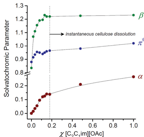
Fig. 7 The influence of solvent composition on the Kamlet–Taft empirical solvation parameters \alpha , \beta and \pi^* , for [C_2C_1im][OAc] –1,3-dimethyl-2-imidazolidinone (DMI) solvents. Adapted from ref. 8 with permission from the Royal Society of Chemistry.
