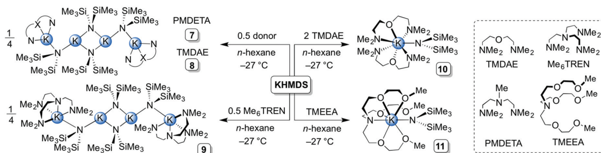
Scheme 2 Synthesis of tetranuclear [(\text{KHMDS})_2(\text{PMDETA-KHMDS})_2] 7 , [(\text{KHMDS})_2(\text{TMDAE-KHMDS})_2] 8 and [(\text{KHMDS})_2(\text{Me}_6\text{TREN-KHMDS})_2] 9 , and monomeric [\text{KHMDS}(\text{TMDAE})_2] 10 and [\text{KHMDS}(\text{TMEEA})] 11 .
