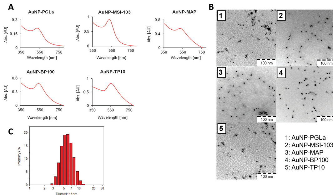
Fig. 2 (A) UV-VIS spectra of PFP. All conjugates show a characteristic red color, and plasmon resonance with a maximum around 525–555 nm. (B) TEM images of PFP, showing a homogeneous size distribution (scale bar = 100 nm) and (C) DLS data showing a series of measurements illustrating a narrow size distribution of functionalized gold nanoparticles (here shown for PGLa) with a mean diameter of around 5–7 nm measured as described previously.
