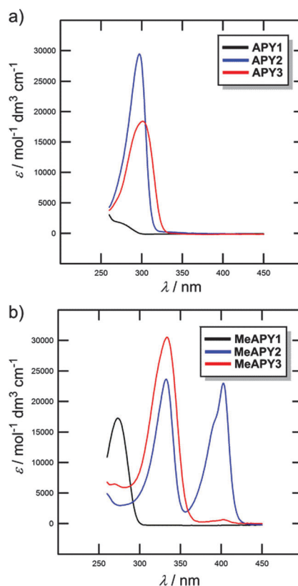
Fig. 3 UV/Vis absorption spectra of APY1–3 (a) and MeAPY1–3 (b) measured in DMSO ( c = 2 \times 10^{-5} M)
