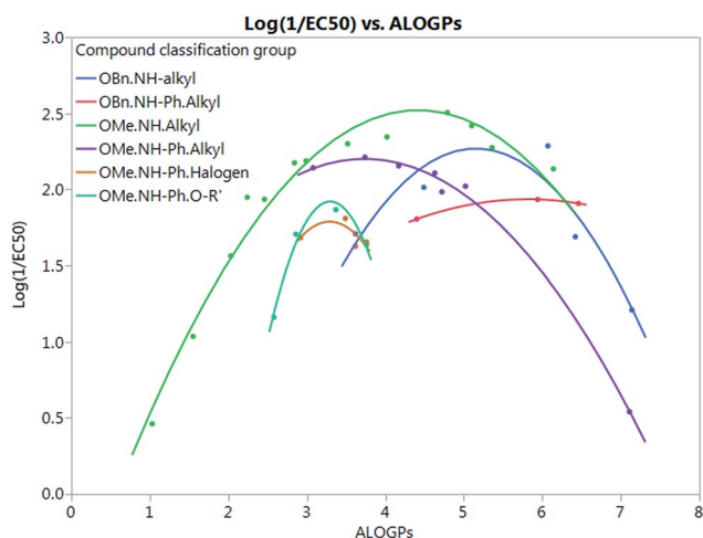
Fig. 7 Quadratic fits for all types of compound grouping, excludes groups with less than 3 points, showing behaviour consistent with a parabolic dependence on log P but with differing optimum values of log P suggesting that other aspects of the mechanism may be more significant in these cases. Groups are classified by the following substituents; R 4 -R 5 -R 6 (R-type).
