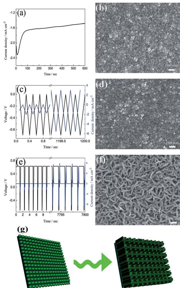
Fig. 1 The current-time responses and the corresponding SEM images for electrodeposited \text{WO}_3 films on ITO glasses: (a and b) continuous deposition, (c and d) pulsed electrodeposition without interval time, (e and f) pulsed electrodeposition with 1.1 s interval time between each pulse. (g) The formation process of porous and interconnecting flaky \text{WO}_3 film.
