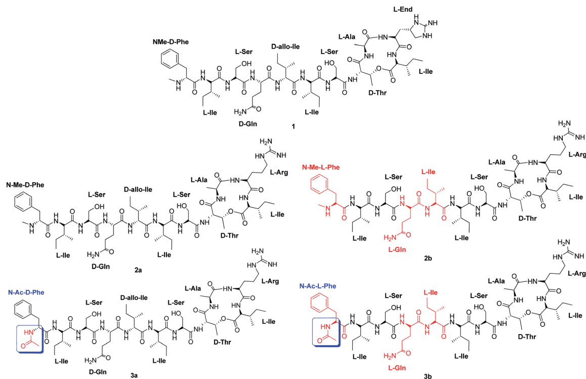
Fig. 1 Structure of teixobactin. (1) Structure of teixobactin analogue (2a) with D-amino acids at the tail and a N(Me)-terminal. 6,9 Structure of teixobactin analogue (2b) with L-amino acids at the tail and a N(Me)-terminal (new analogue). Structure of teixobactin analogue (3a) with D-amino acids at the tail and a N(Ac)-terminal (new analogue). Structure of teixobactin analogue (3b) with L-amino acids at the tail and a N(Ac)-terminal. 11
