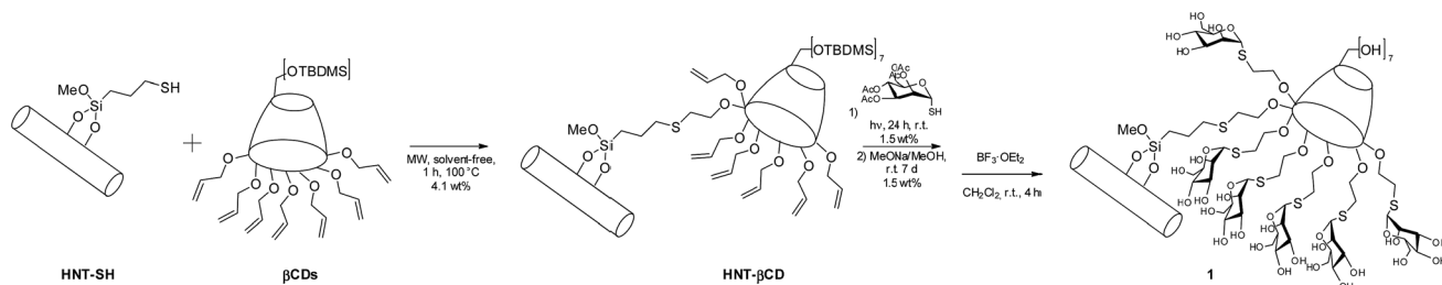
Fig. 3 Synthesis of compound 1.
