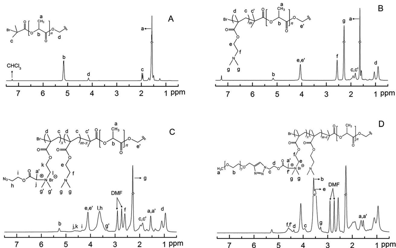
Fig. 1 ^1\text{H} NMR spectra of (A) PLLA-diBr and (B) D-PLLA-D in \text{CDCl}_3 , (C) D-PLLA-D@Q and (D) D-PLLA-D@QPPEG-2 in d\text{-DMF} .
