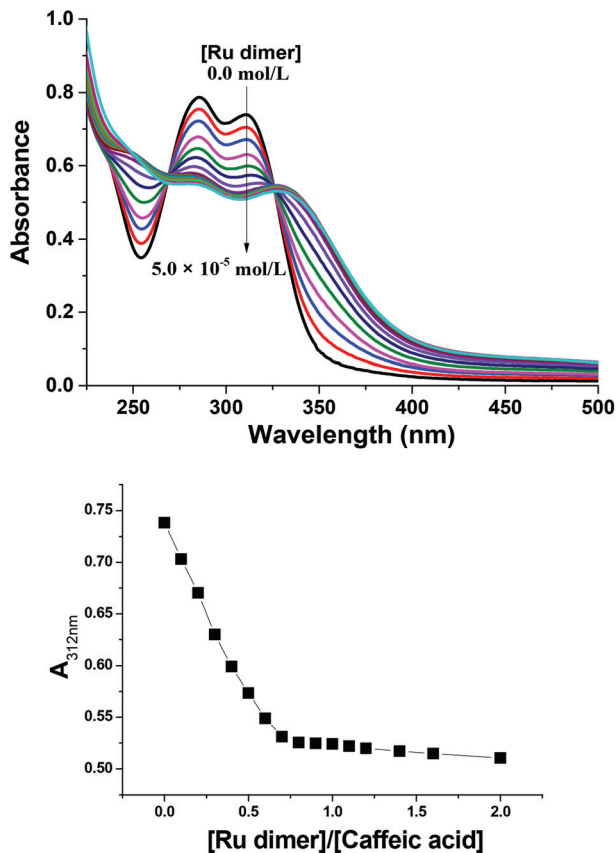
Fig. 6 Top: UV-vis spectra for the reaction of various concentrations of Ru dimer with caffeic acid-modified chitosan, [caffeic acid in caffeic acid-modified chitosan] = 5.0 \times 10^{-5} mol L -1 , in water. Bottom: Changes in absorbance at 312 nm at various concentrations of Ru dimer with caffeic acid-modified chitosan.
