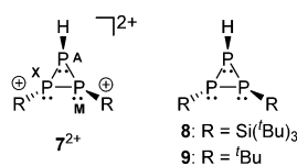
Fig. 2 Substituent arrangement in cyclo -triphenylphosphanes 7^{2+} , 8 and 9 .
