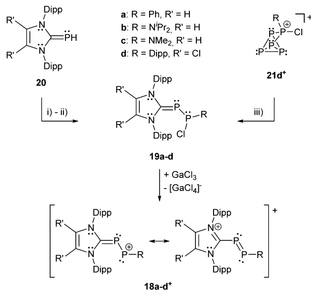
Scheme 7 Two different approaches for the synthesis of NHC stabilized chlorodiphosphenes 19a-d comprising bonding motif B. For 19a,b : (i) +\text{R}_2\text{PCl}_2 , +\text{DABCO} , -\text{DABCO}\cdot\text{HCl} ; for 19c : (ii) +2\text{PCl}(\text{NMe}_2)_2 , +\text{DABCO} , -\text{DABCO}\cdot\text{HCl} , -\text{P}(\text{NMe}_2)_3 ; for 19d : (iii) +3\text{1,3-bis(2,6-diisopropylphenyl)-4,5-dichloro-imidazole-2-ylidene} , -\text{5 +. Subsequent chloride abstraction yields polarized cationic diphosphenes 18a-d + . Only two resonance structures that indicate the polarization of 18a-d + are shown.
