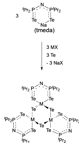
Scheme 3 General synthesis of [\text{Ga}(\mu\text{-Te})\{\text{N}(\text{Te}^i\text{Pr}_2)_2\}]_3 ( \text{M} = \text{Ga} , \text{X} = \text{I} ) and [\text{In}(\mu\text{-Te})\{\text{N}(\text{Te}^i\text{Pr}_2)_2\}]_3 ( \text{M} = \text{In} , \text{X} = \text{Cl} ).
